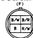
FR-02 CONNECTOR BETWEEN FRONT(F) AND REAR(R) HARNESS
