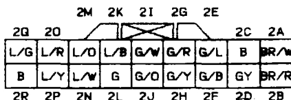
FEM-01 CONNECTOR BETWEEN FRONT(F) AND EMISSION(EM) HARNESS
