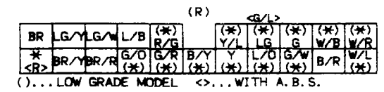
FDR-01 CONNECTOR BETWEEN FRONT(F) AND NO. 1 DOOR(DR1) HARNESS(L. H.)
