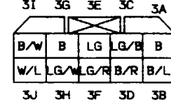
FE-02 CONNECTOR BETWEEN FRONT(F) AND ENGINE(E) HARNESS
