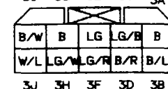
EM-03 EMISSION CONTROL UNIT (EM)
