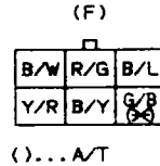
FE-02 CONNECTOR BETWEEN FRONT(F) AND ENGINE(E) HARNESS
