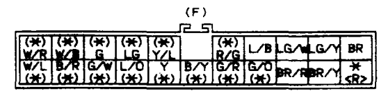
FR-01 CONNECTOR BETWEEN FRONT(F) AND REAR(R) HARNESS
