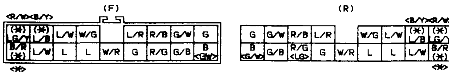
FR-02 CONNECTOR BETWEEN FRONT(F) AND REAR(R) HARNESS
