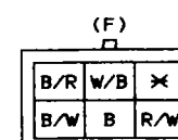
FE-03 CONNECTOR BETWEEN FRONT(F) AND ENGINE(E) HARNESS
