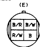
FE-05 CONNECTOR BETWEEN FRONT(F) AND ENGINE(E) HARNESS
