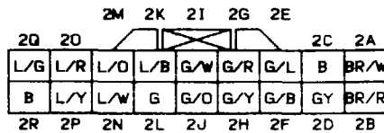
EM-31 EMISSION CONTROL UNIT(EM)
