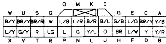
F-36 COIL WITH IGNITER(L)(F)
