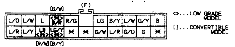
FC-01 CONNECTOR BETWEEN FRONT (F) AND CLUSTER SWITCH (CR2) HARNESS
