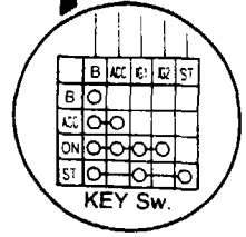
Ignition Switch
