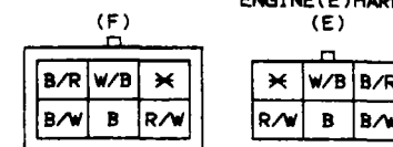
FR-02 CONNECTOR BETWEEN FRONT(F) AND REAR(R) HARNESS
